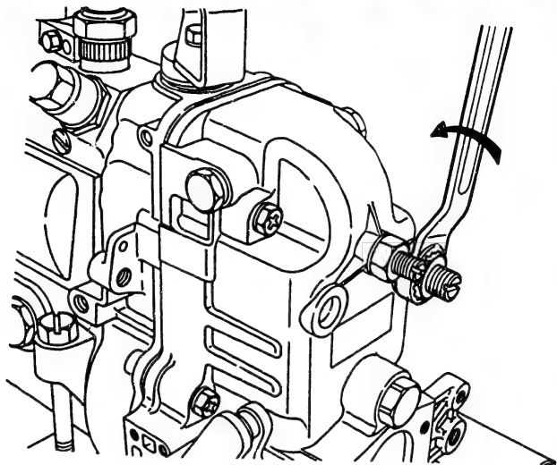
Fig. 22 Loosening locknut
